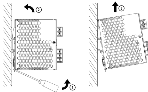
Fig. 2.2 Dismounting
